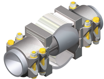
230 kV Aluminum Bolted Couplers
