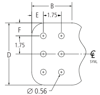
Pad Detail 3
