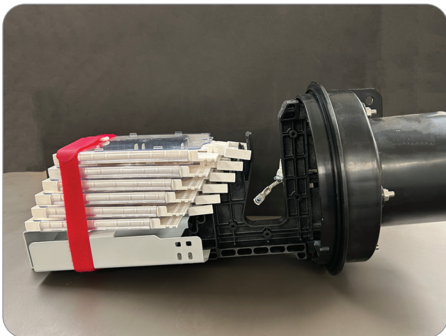
Figure 18 – Apex X-2S Trays in FOSC C
