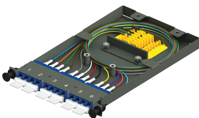
MXHD-SP-1A1-N-N12-LCUBU MXHD Splice Cassette, 12F, SM G.657.A1, 900 µm TB Pigtails, LC/UPC Blue
