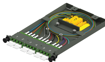
MXHD-SP-1A1-N-N12-LCAGN MXHD Splice Cassette, 12F, SM G.657.A1, 900 µm TB Pigtails, LC/APC Green
