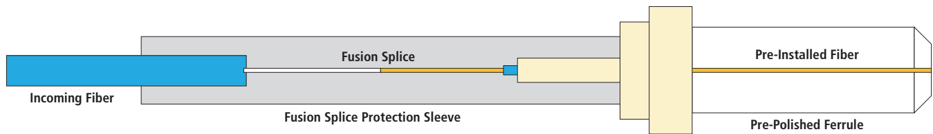
Figure 2—FUSEConnect SC, FC, LC and ST Connectors
