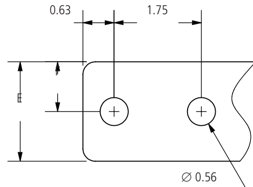
Pad Detail 1
