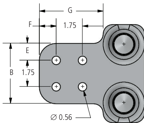
Pad Detail 1
