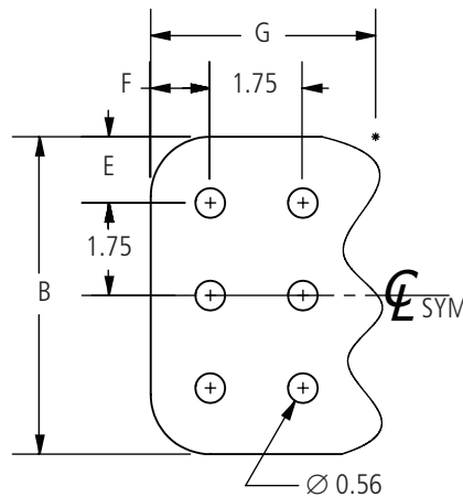
Pad Detail 2
