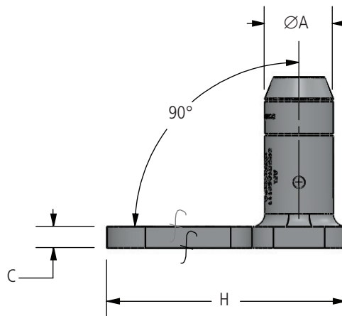
Pad Detail 2
